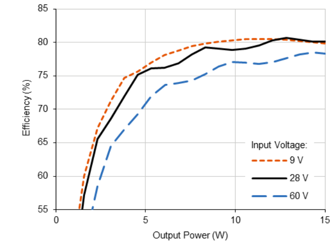
4.1.2 VXR15-280505D Efficiency (Typical, 25 °C)
