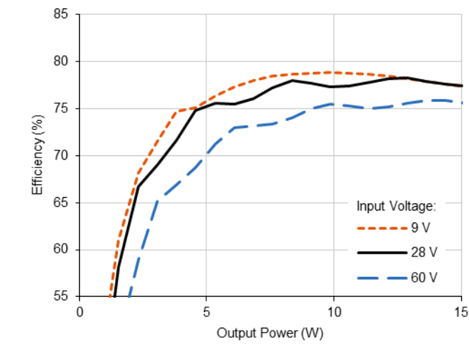
4.1.1 VXR15-283R33R3D Efficiency (Typical, 25 °C)
