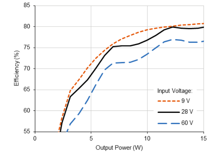
4.1.3 VXR15-281212D Efficiency (Typical, 25 °C)
