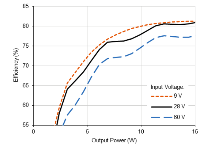
4.1.4 VXR15-281515D Efficiency (Typical, 25 °C)
